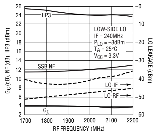
Conversion Gain, IIP3, SSB NF and LO Leakage vs RF Frequency
